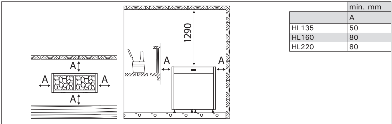
Minimum safety distances (all dimensions in millimeters)
