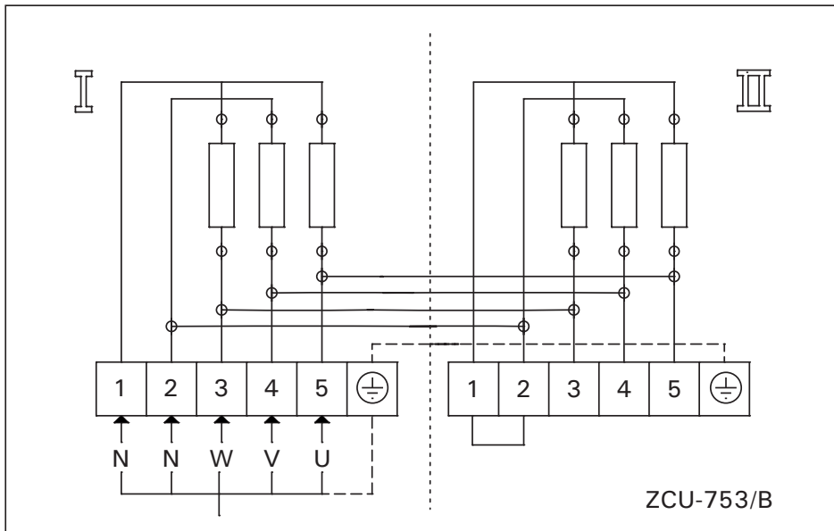
Electrical connections of heater HL135/160 Pro
