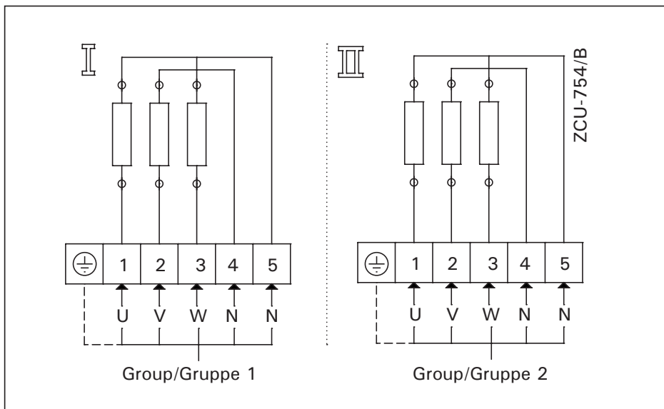
Electrical connections of heater HL220 Pro
