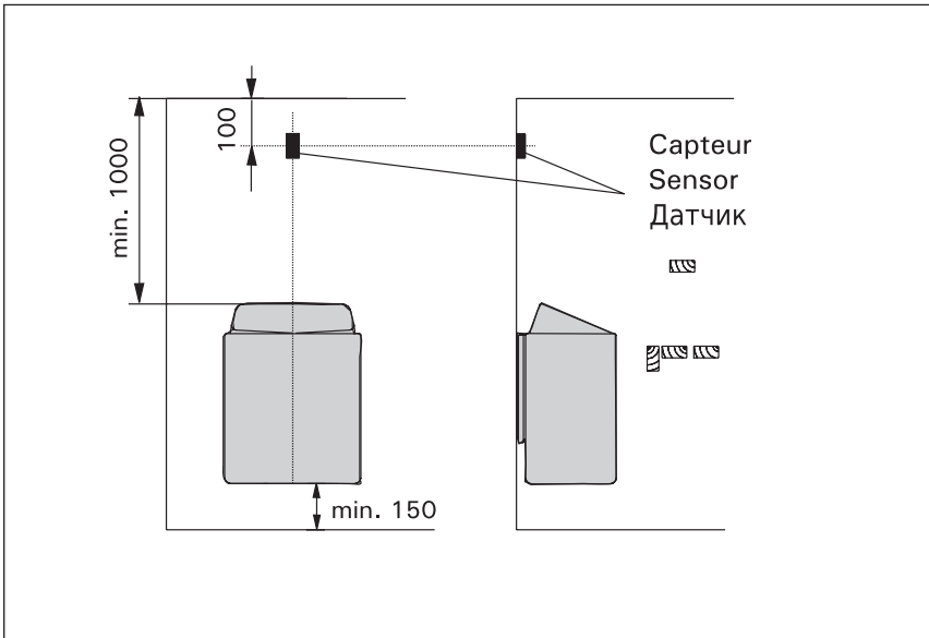
The place of the sensor box of the control unit connection with wall-mounted heaters.
