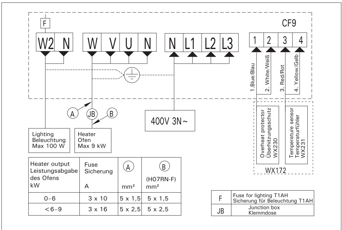
Electrical connections for the heaters, as well as for the control unit CF9
