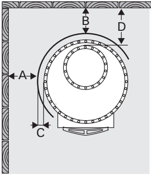
Legend Protection Supplies (all dimensions in millimeters)
