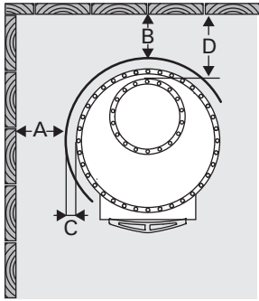
Legend Protection Supplies (all dimensions in millimeters)
