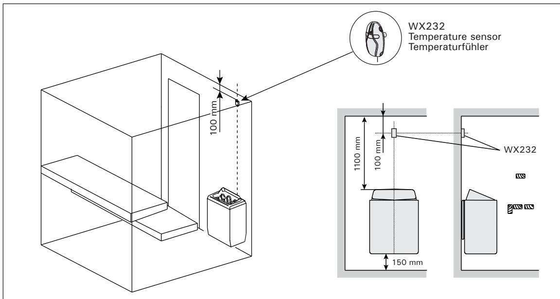
The place of the temperature sensor in connection with wall-mounted heaters
