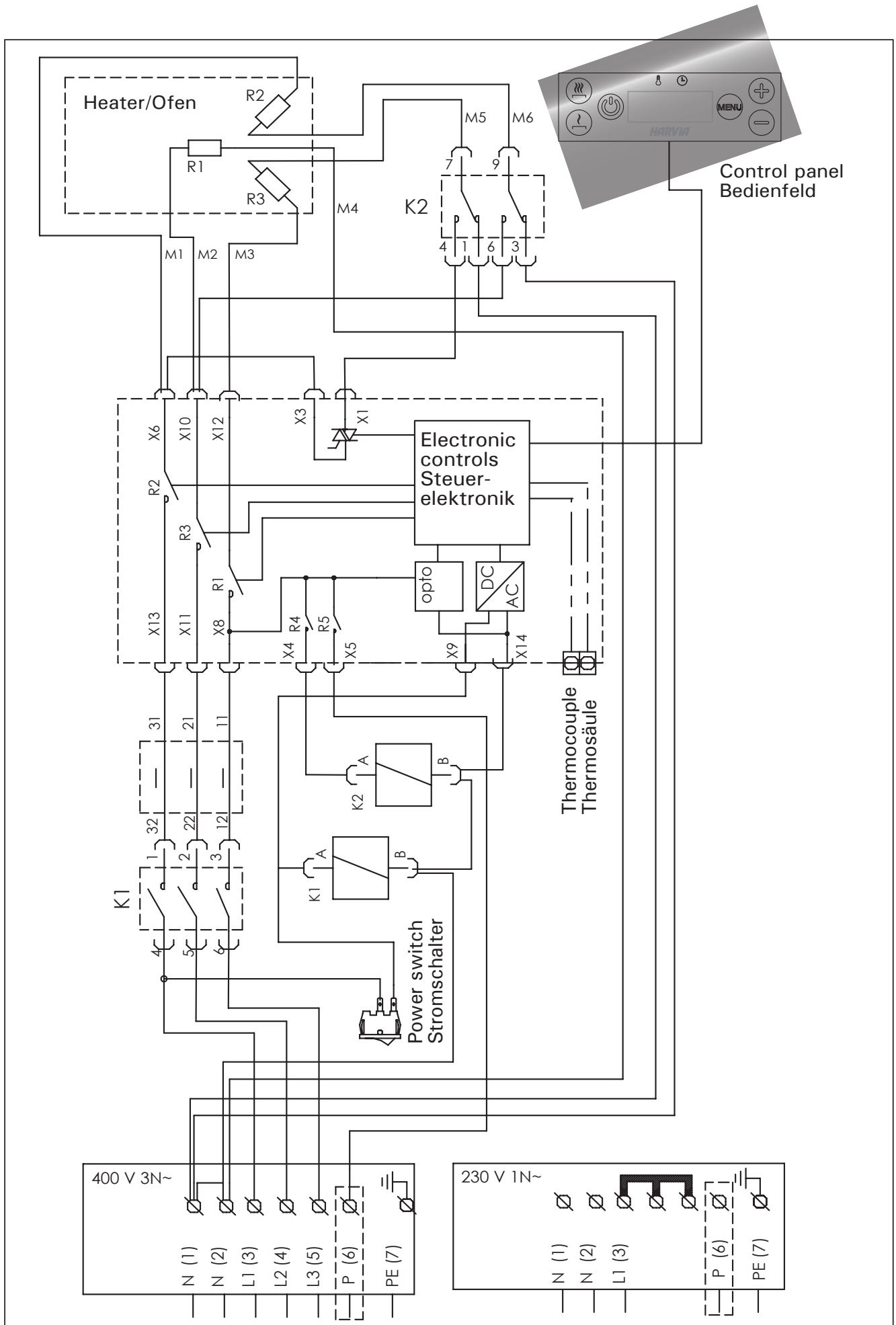
Electrical connections of heater
