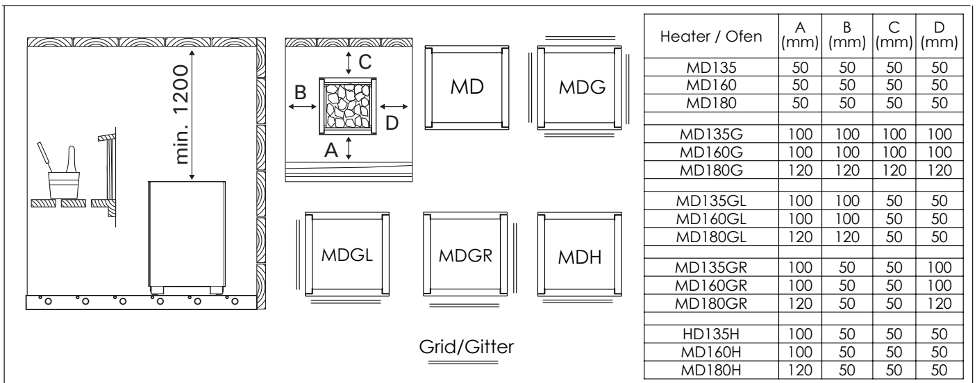
Minimum safety distances (all dimensions in millimeters)
